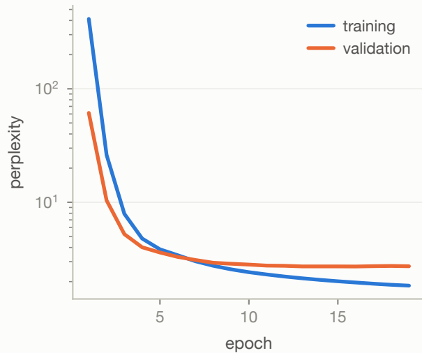
Perplexity
