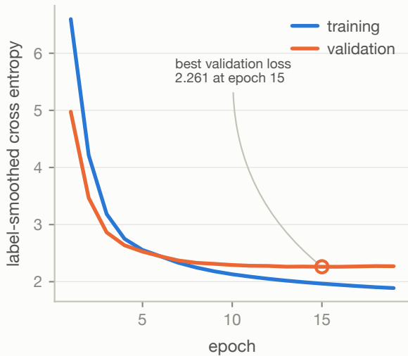
Loss
