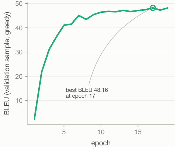
Translation quality
