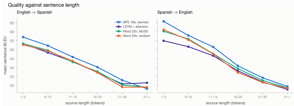
Figure 16: Sentence-level BLEU stratified by source length. This figure tests the central architectural claim: a recurrent model must carry information across a number of sequential steps proportional to sentence length, whereas in a transformer every pair of positions is one attention hop apart, so the recurrent model should degrade faster as sentences lengthen.
