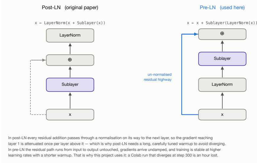
Figure 10: Where to put the layer normalisation, and why it changes training stability.
