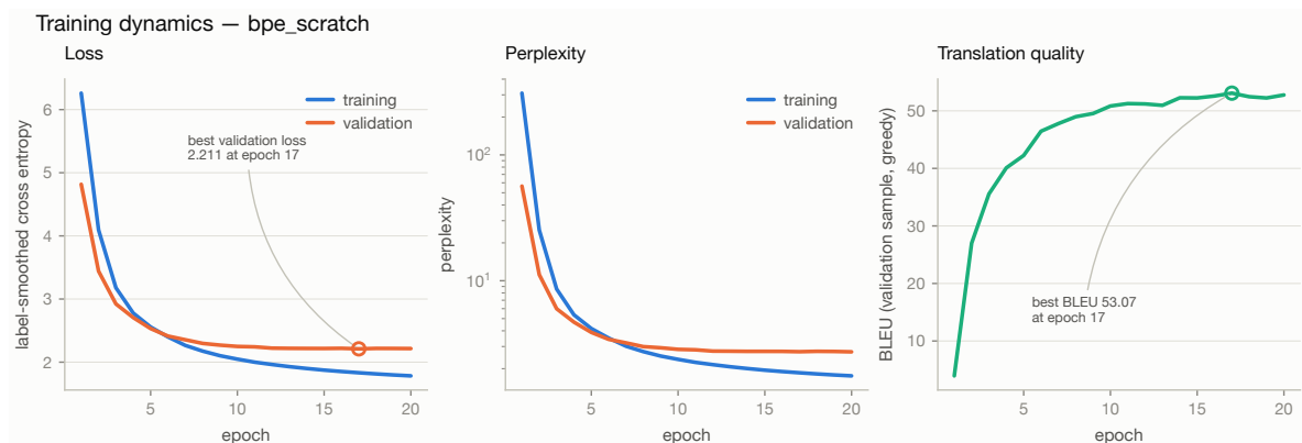
Figure 12: Training and validation curves for the primary model. Loss and BLEU are shown on separate axes rather than as a dual-axis chart: two y -scales on one frame invite comparison of slopes that share no units, and the apparent crossing point would be an artefact of scaling.
