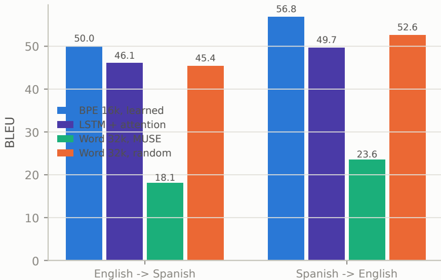
BLEU on the held-out test set
