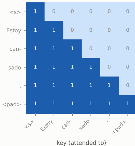
Causal mask
