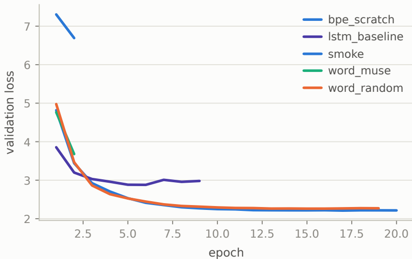
Validation loss
