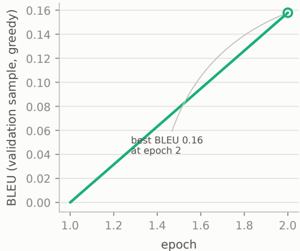
Translation quality
