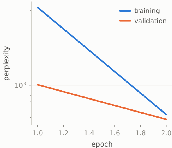
Perplexity
