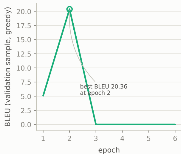
Translation quality
