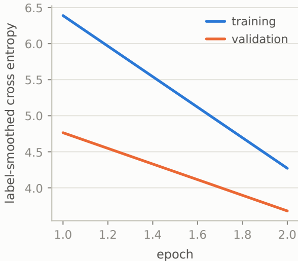
Loss
