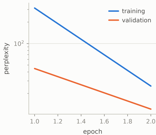
Perplexity
