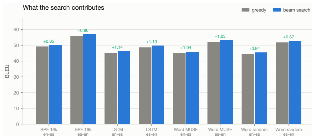
Figure 18: What the search contributes: BLEU under greedy decoding against beam search. A large gap means the model’s single-best token is often wrong even when its distribution is right.
