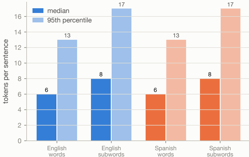
Segmentation lengthens sequences
