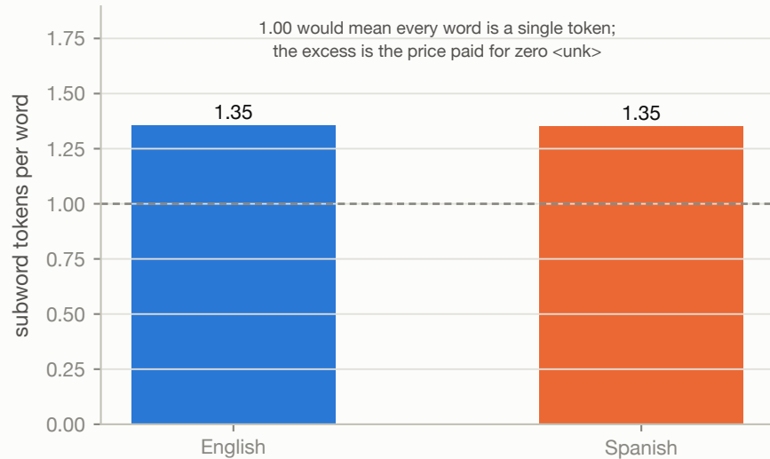
Fertility of the 16k joint BPE model
