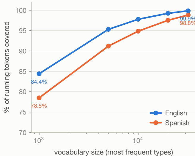
Coverage of running text
