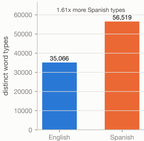
Vocabulary size
