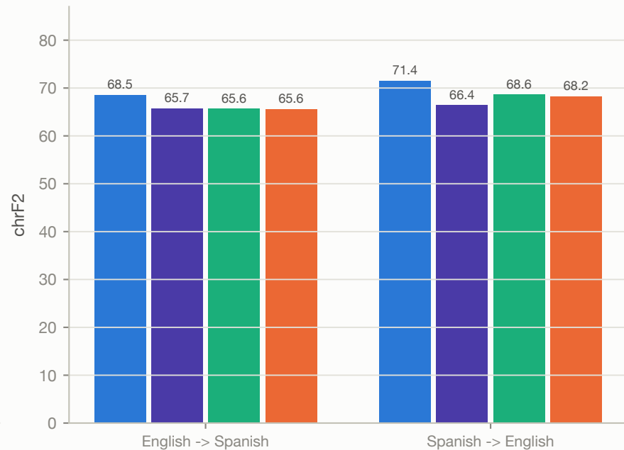
chrF2 on the held-out test set
