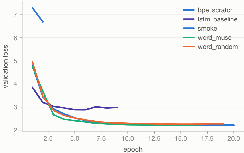
Validation loss
