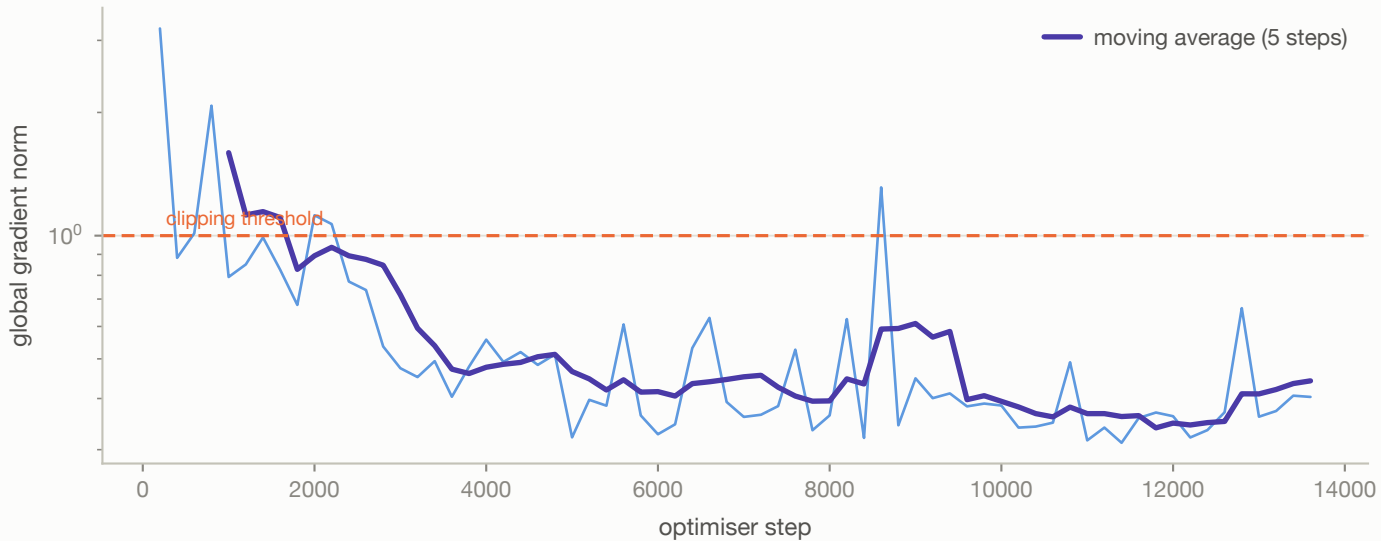
Gradient norms and the clipping threshold
