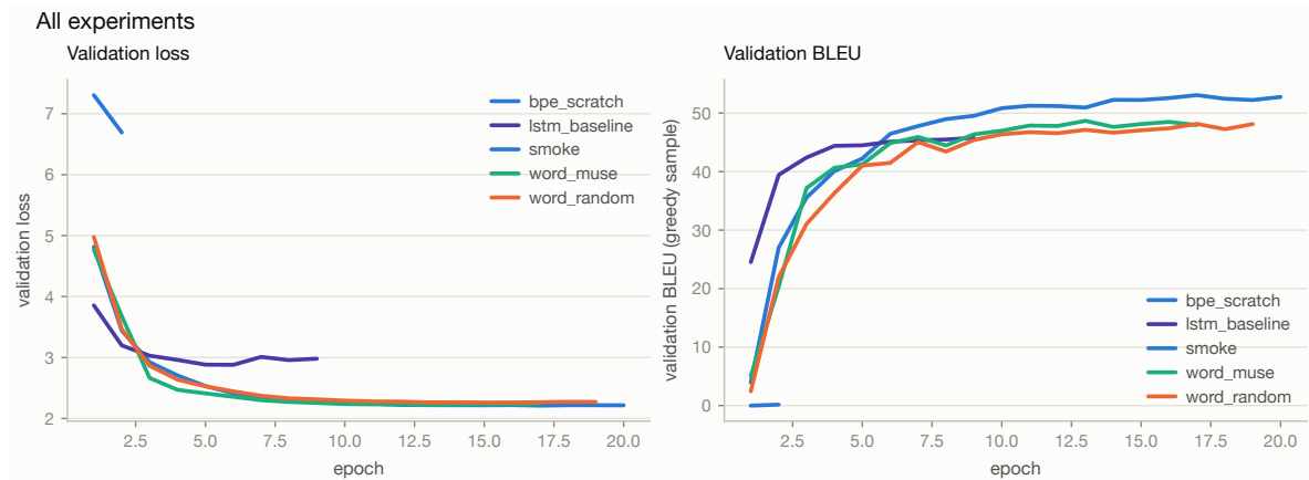
Figure 13: Validation loss and BLEU for all four systems. The recurrent baseline reaches a given BLEU in fewer epochs than the transformers but plateaus lower and earlier, stopping at epoch 9 against 17–20 for the transformers.
