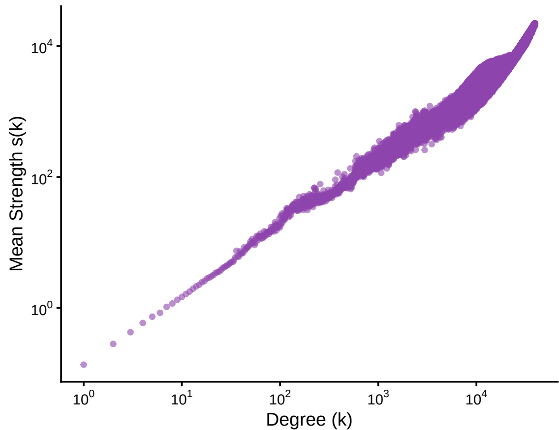
Mean Strength vs Degree – network_purple
