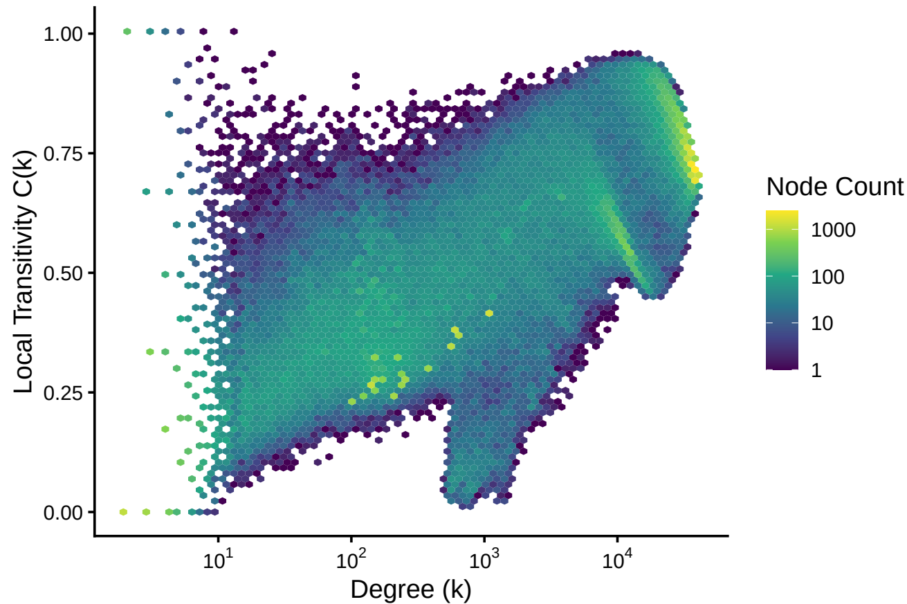
Transitivity vs Degree – network_purple
