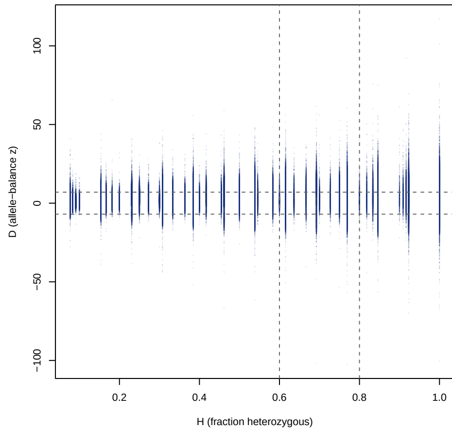
HDplot, 300K random SNPs
