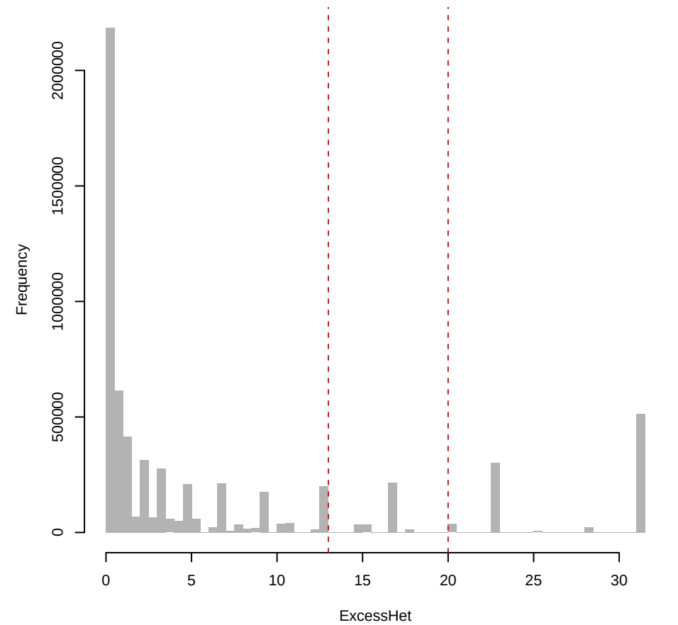
ExcessHet (max 31.0 at n = 13)
