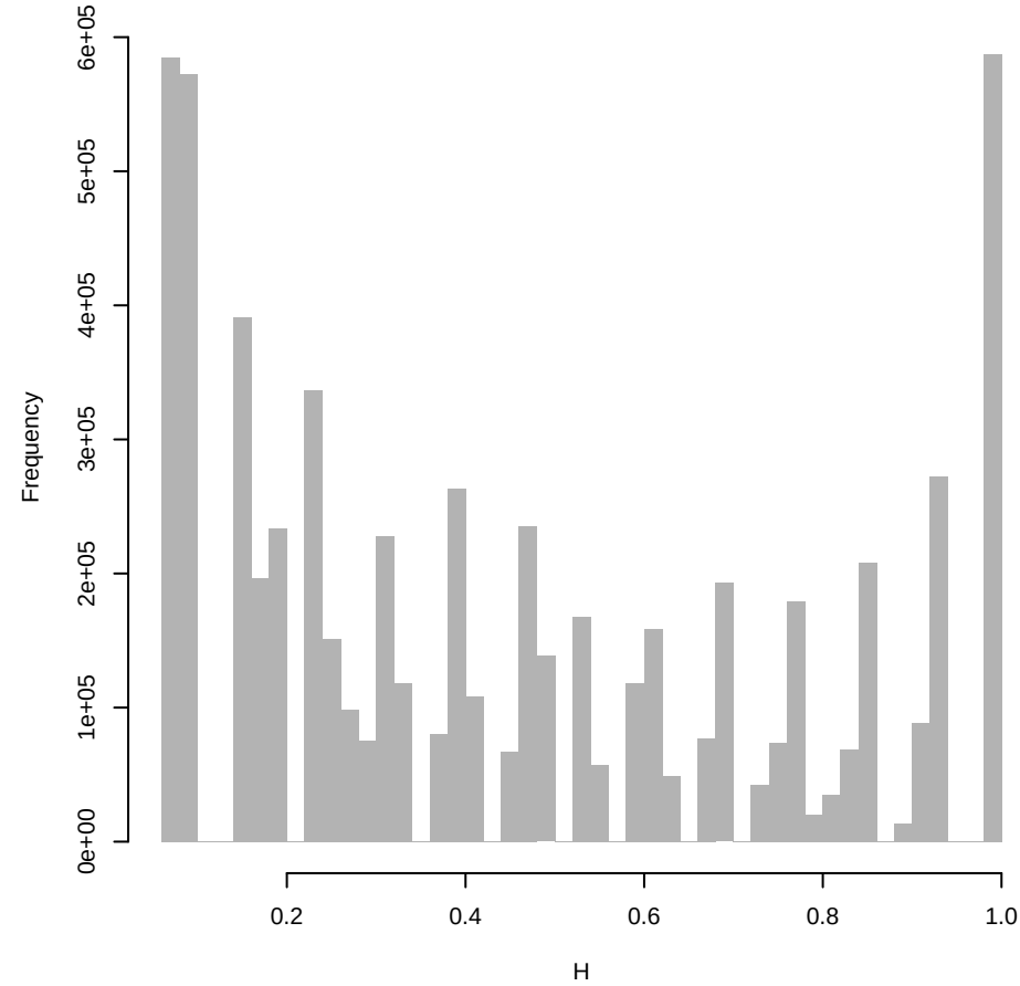
H, all biallelic SNPs
