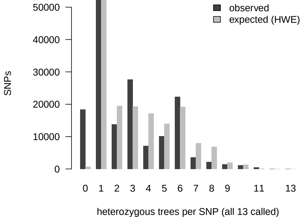
d09_item3_masked_v2_gtfilt: observed vs HWE
