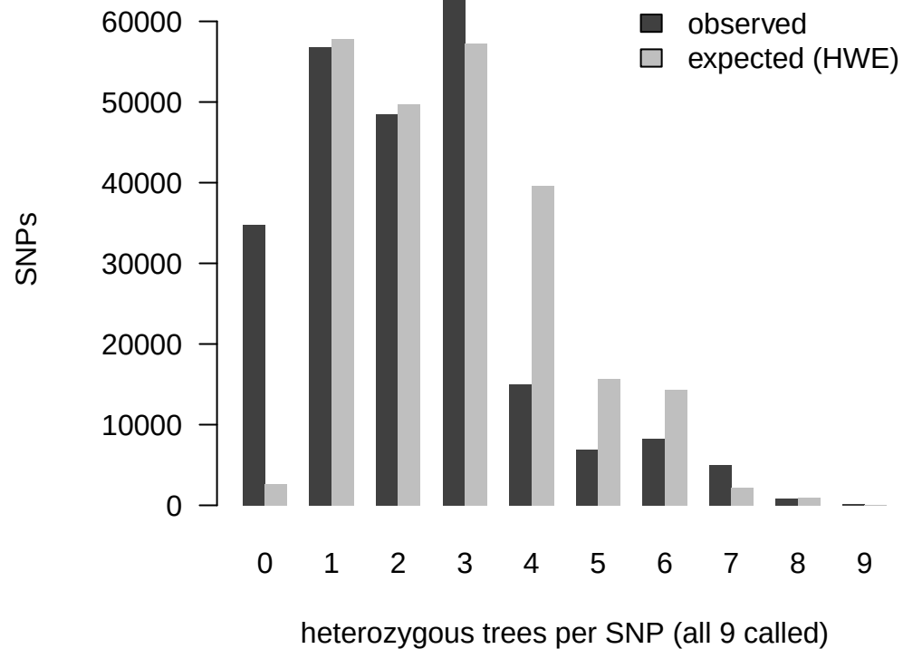
d20_v2_DP3_p1e-2: observed vs HWE
