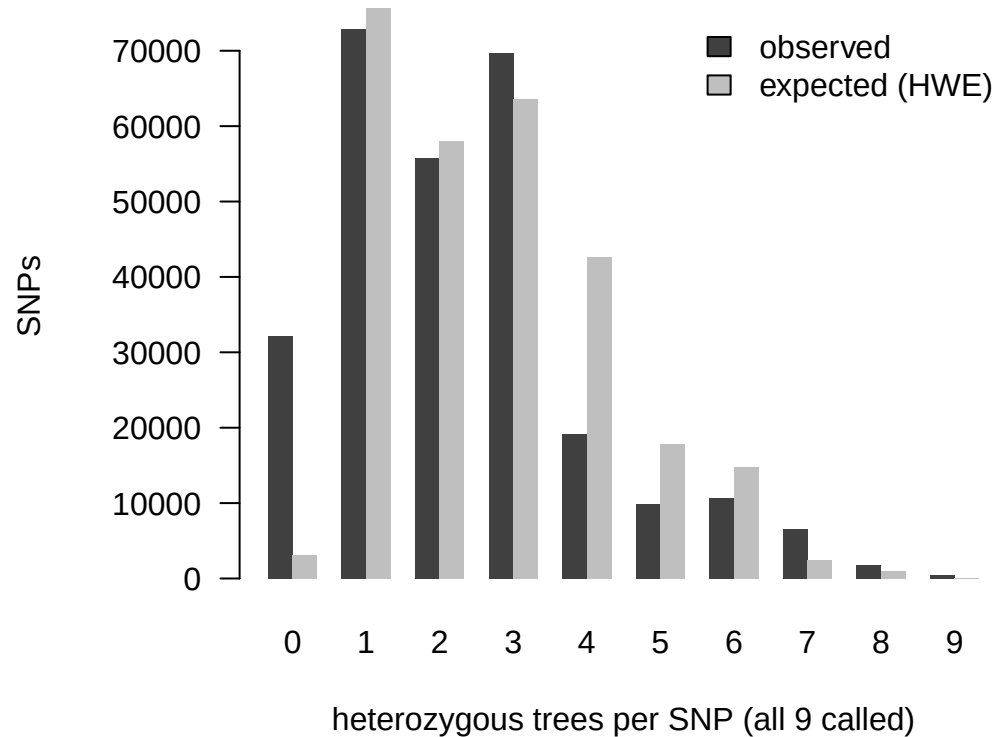
d20_v2_G1_p1e-4: observed vs HWE
