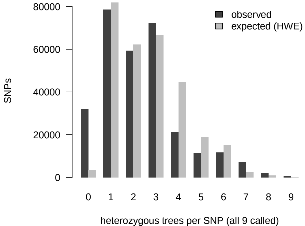
d20_v2_G1_p1e-5: observed vs HWE
