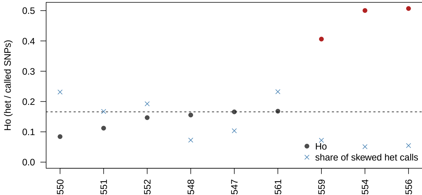
d20_v2_G1_p1e-2: Ho per tree (red = >3 MAD)
