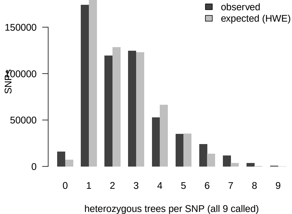
d20_mask_h75: observed vs HWE
