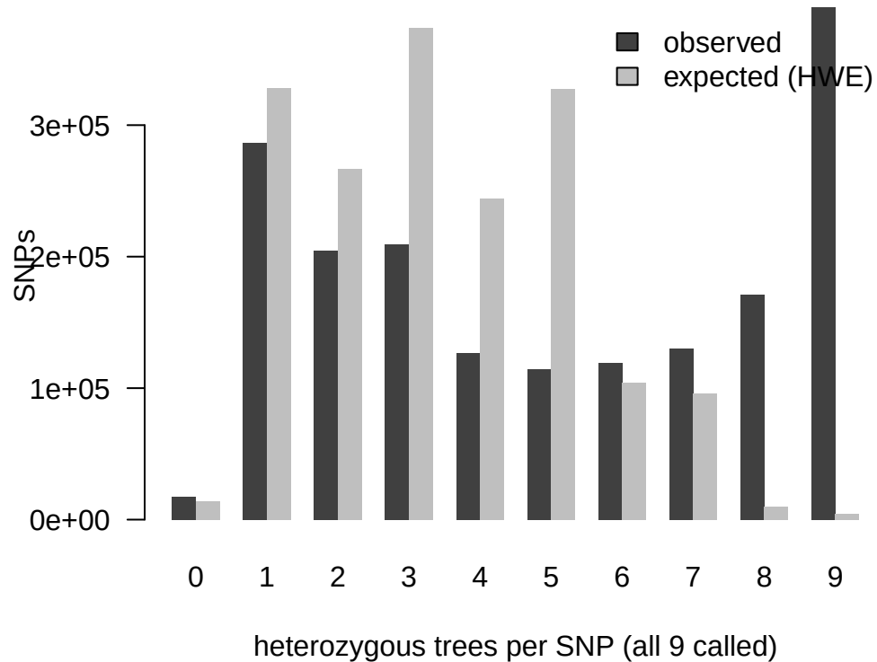
d20_unmasked: observed vs HWE
