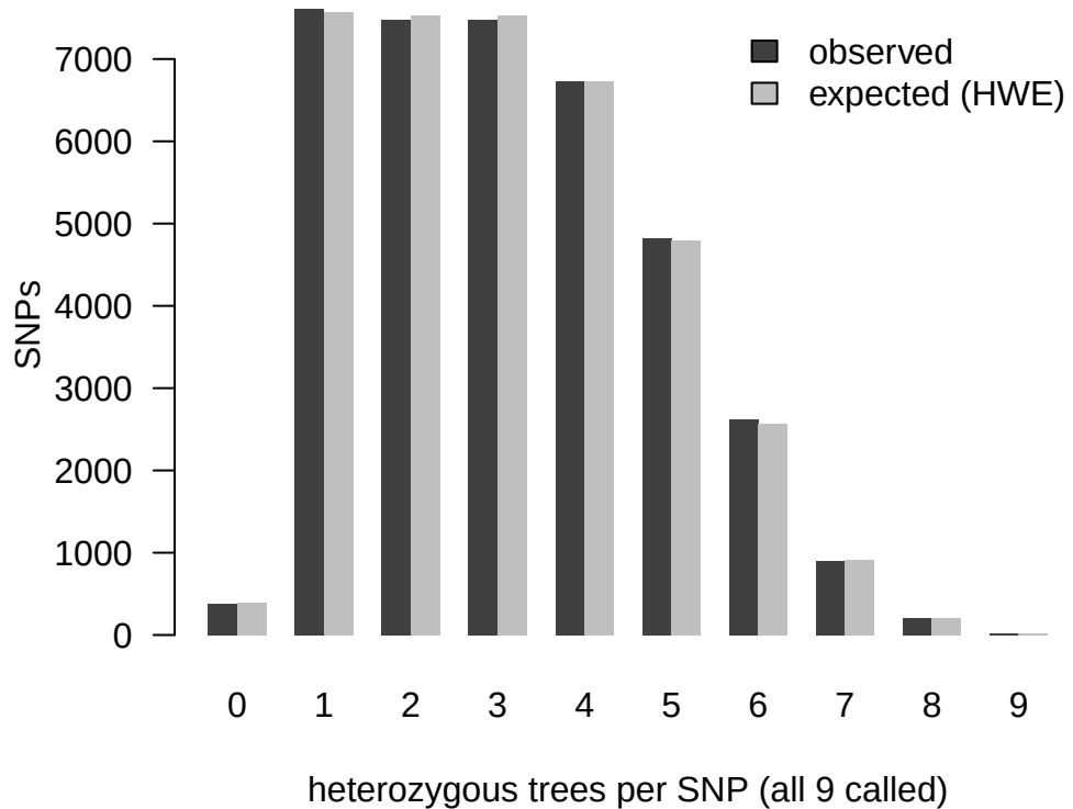
sim_hwe: observed vs HWE
