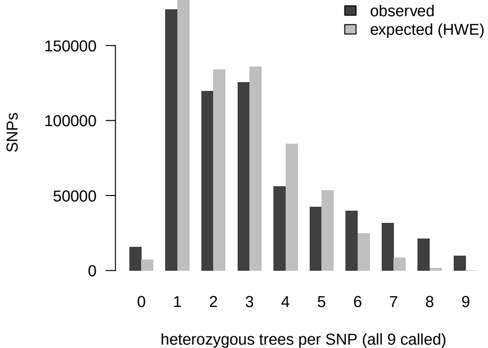
d20_mask_current: observed vs HWE
