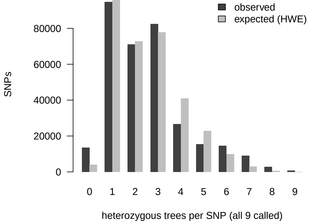
d20_mask_win1kb: observed vs HWE
