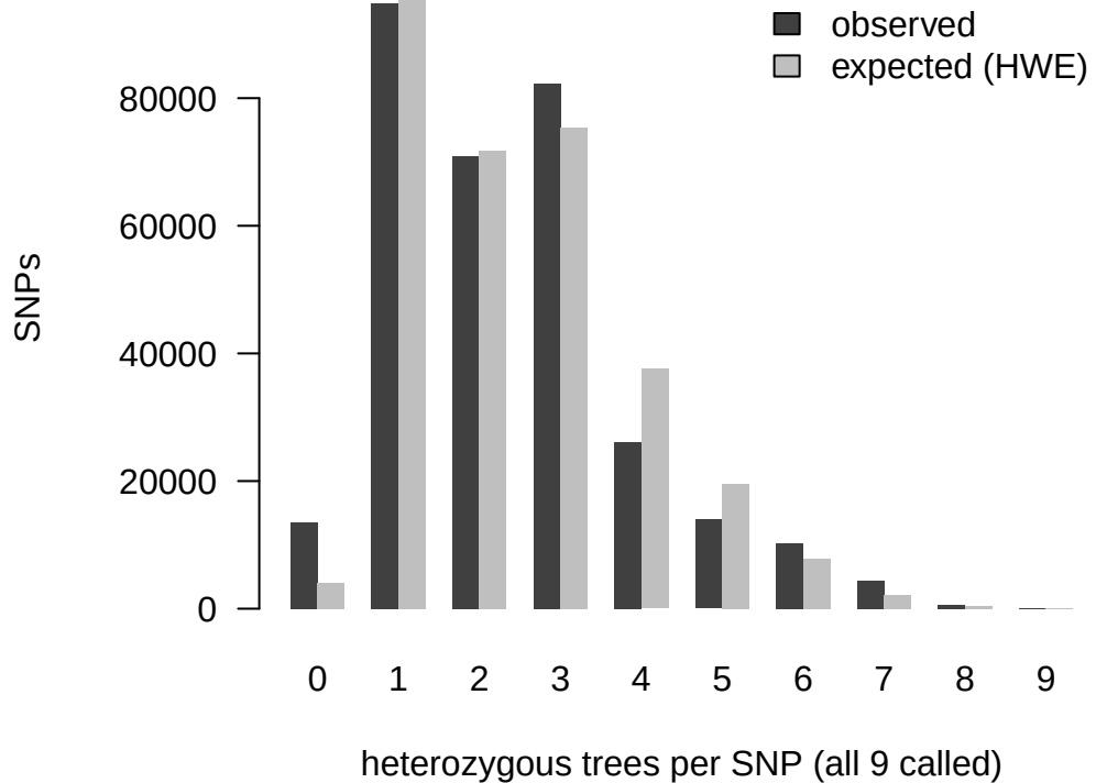
d20_mask_win1kb_h75: observed vs HWE
