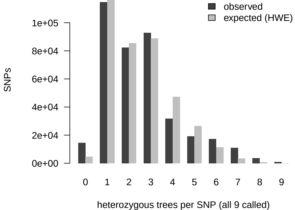
d20_mask_win500: observed vs HWE
