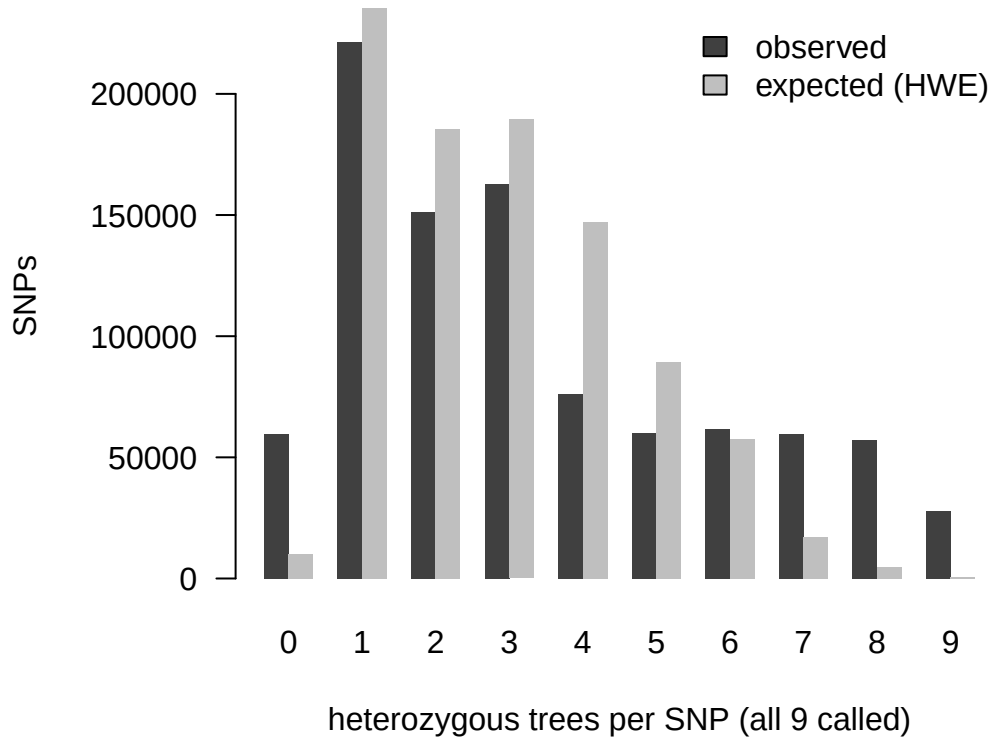
native_d20trees_masked: observed vs HWE
