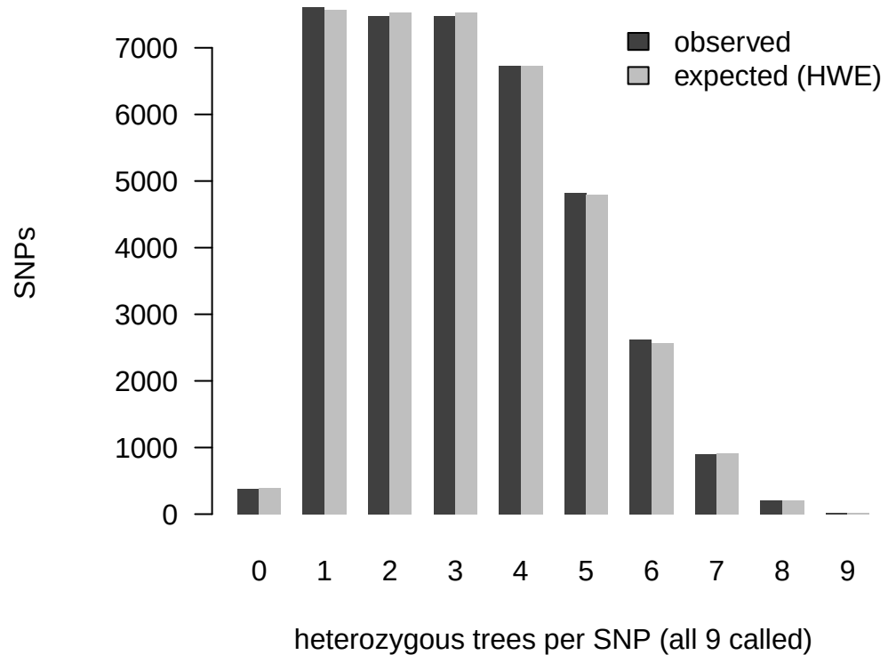
sim_hwe: observed vs HWE
