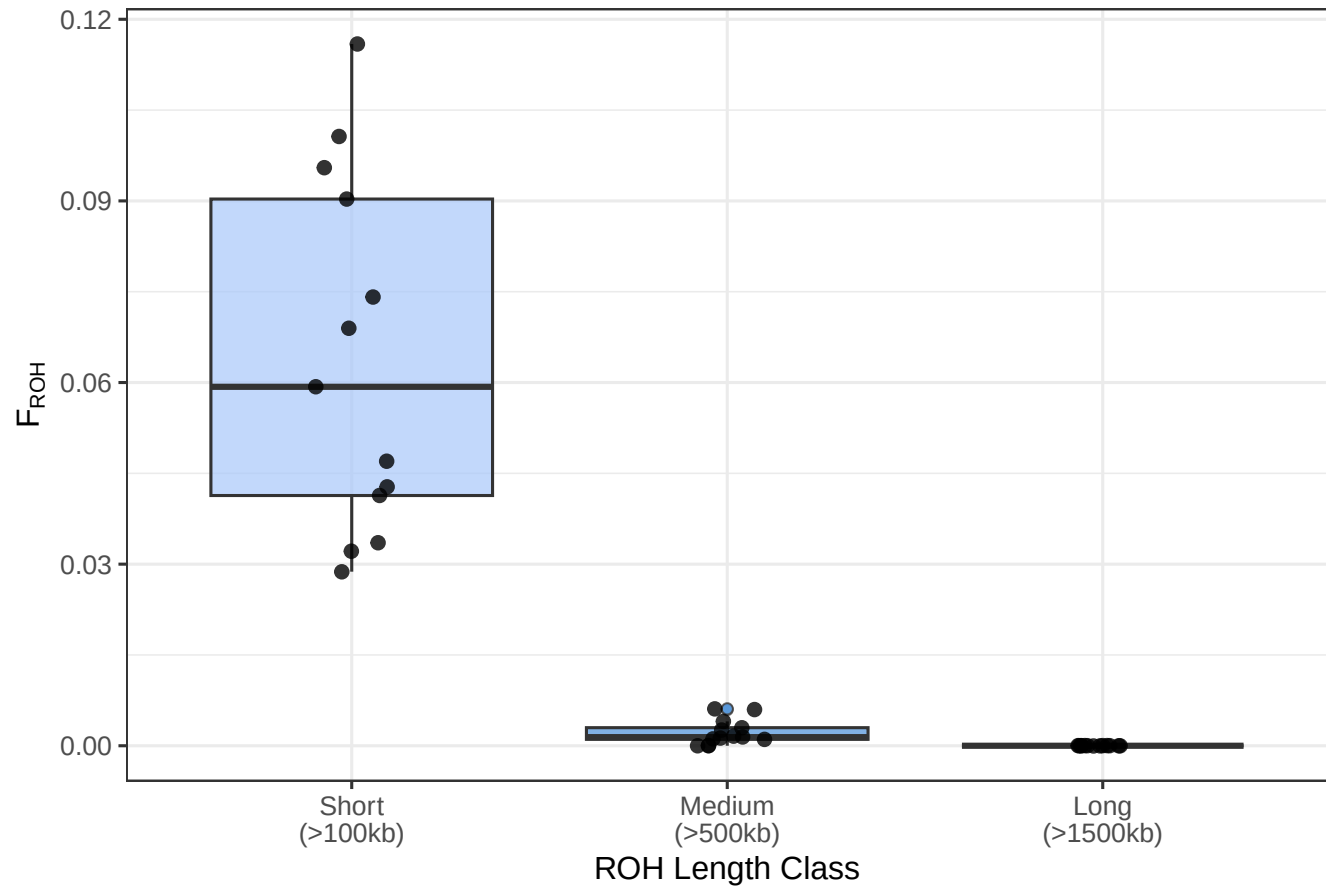
F_ROH Distribution by ROH Length Class – d09
