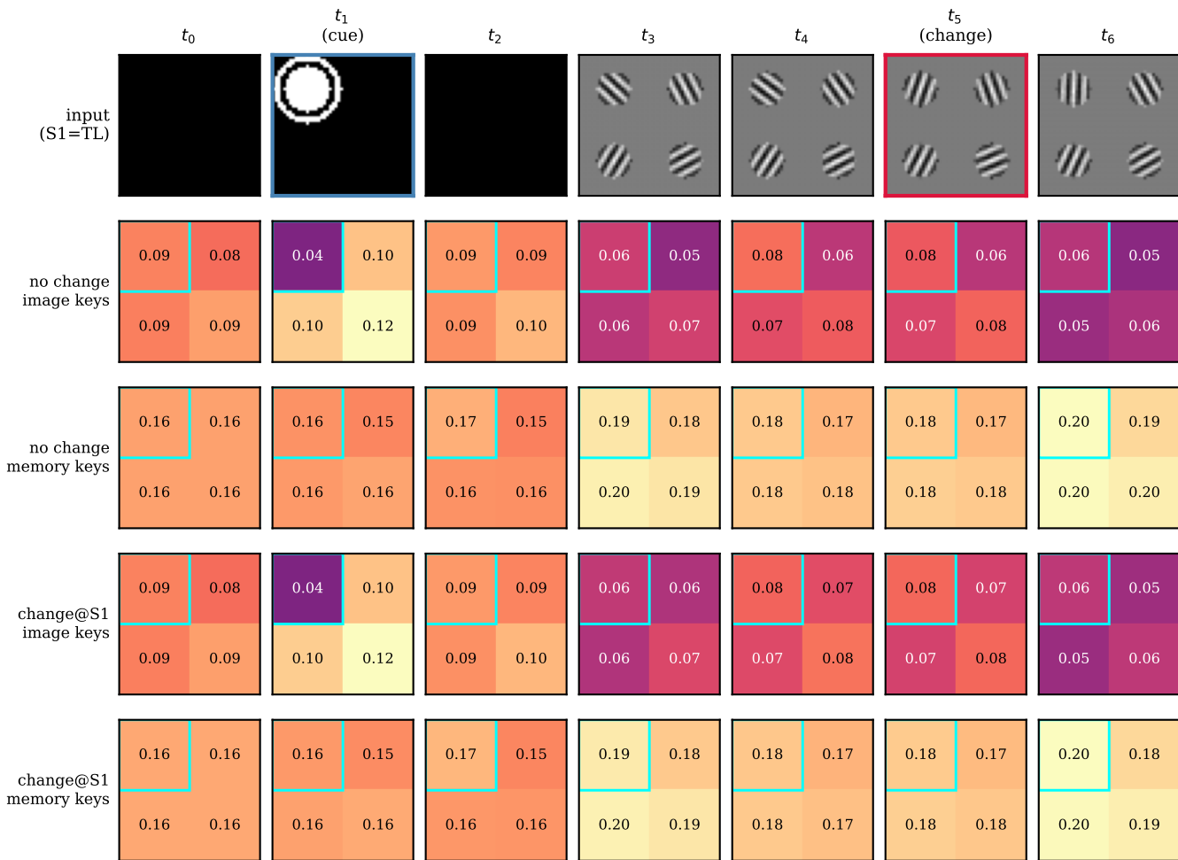
Cross-attention (image+memory) — attention maps, 100% cue at S1 (cyan = cued/changed patch)
