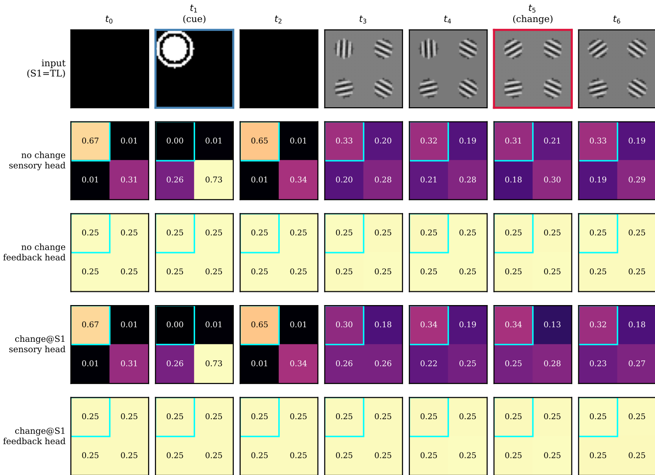
Dual-head (sensory+feedback) — attention maps, 100% cue at S1 (cyan = cued/changed patch)
