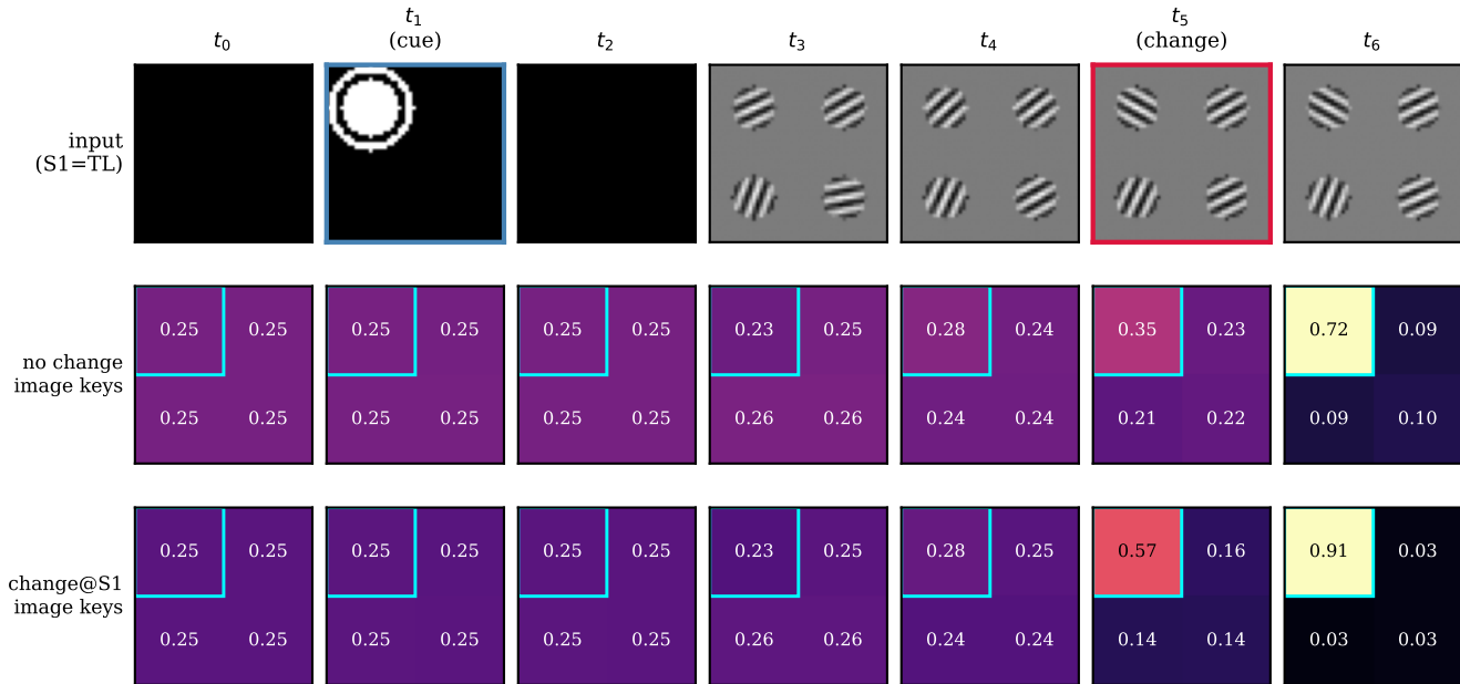
Two stacked xLSTMs — attention maps, 100% cue at S1 (cyan = cued/changed patch)
