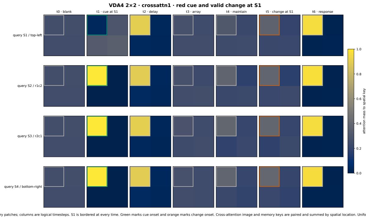
Figure 11: VDA4 cross-attention. Checkpoint-recomputed descriptive measurement; 96 trials. Image and memory keys are paired and summed by spatial location before plotting. The four query rows, seven logical timesteps, and fixed [0, 1] scale match Figure 10.
