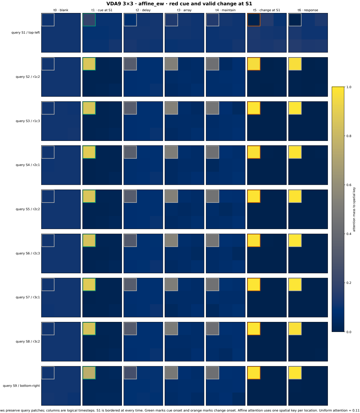
Figure 12: VDA9 affine attention. Checkpoint-recomputed descriptive measurement; 96 trials. Nine query rows and seven logical timesteps are retained. The spatial-key baseline is 1/9 = 0.111 \dots . All cells share the same [0, 1] scale.
