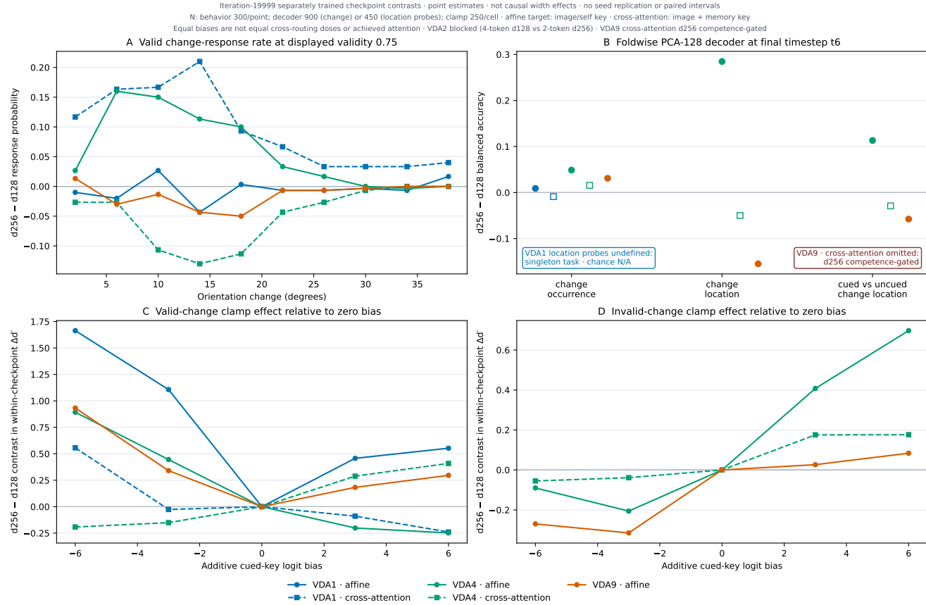
Figure 18: Matched-width checkpoint summary. Checkpoint-recomputed descriptive and model-intervention evidence. Ordinates are d256 minus d128 for separately trained iteration-19999 checkpoints. Panel A shows valid-location response differences at displayed validity 0.75 (300 trials per point); Table 8 gives the absolute constituent curves. Panel B shows t6 foldwise PCA-128 balanced-accuracy differences. Zero, not chance, is Panel B's plotted reference because the ordinate is d256 minus d128; chance values describe the unplotted absolute scores. Binary change occurrence uses all 900 trials (chance 0.5), realized location uses 450 change-present trials (chance 0.25 for VDA4 and 1/9 for VDA9), and cued versus uncued location uses the same 450 trials (chance 0.5). For scale, VDA9 affine d256 realized-location balanced accuracy is 0.499 versus 1/9 = 0.111 chance (d128: 0.654). Structurally chance t0 points are excluded; native warning localization is process-log-derived rather than hash-bound and is omitted conservatively. Panels C and D show the checkpoint contrast in within-checkpoint d' change relative to zero bias (250 trials per cell); Table 9 gives every within-checkpoint constituent. Affine routing biases the cued image key; cross-attention biases that image key and its memory key, so equal biases are not calibrated cross-routing doses or achieved-attention allocations. VDA1 invalid effects are undefined. VDA2 is blocked by a four-token d128 versus two-token d256 geometry mismatch. VDA9 cross-attention is omitted because d256 fails the registered acceptance threshold. Aggregate counts do not preserve trial identities; paired intervals are unavailable.
