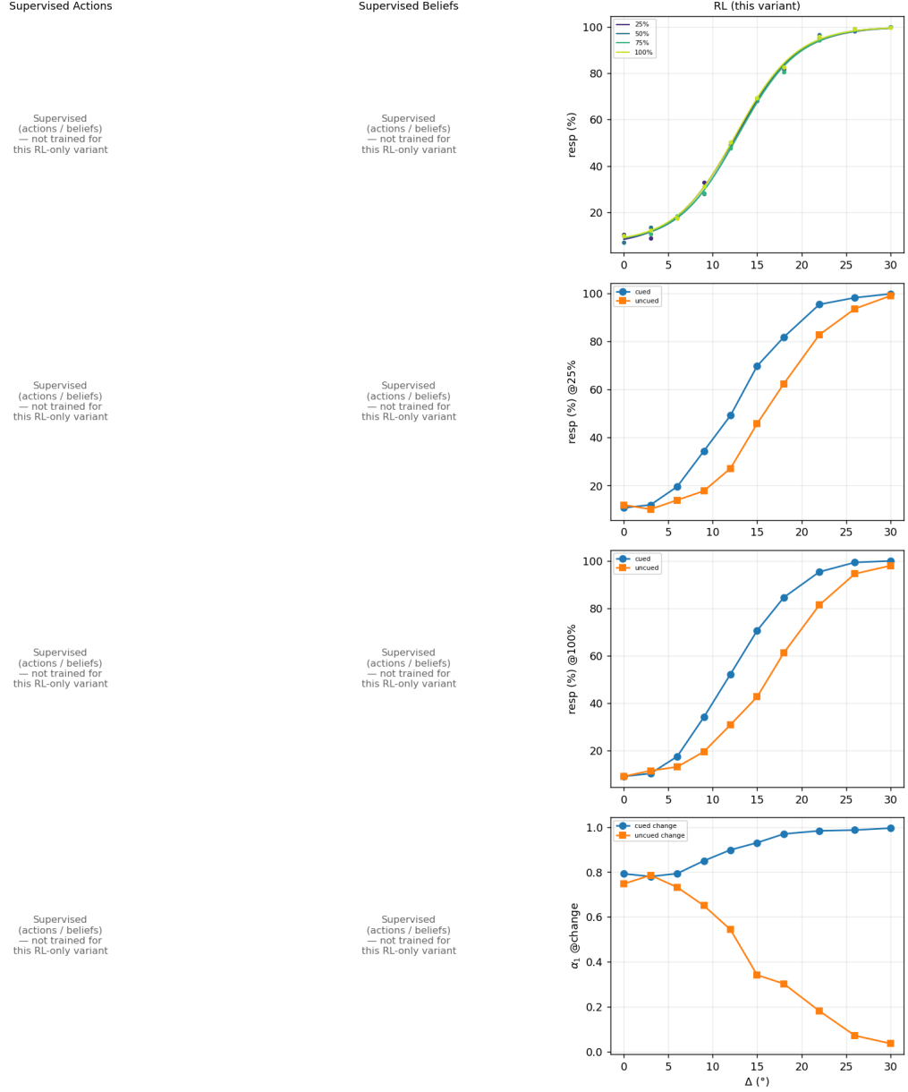
Figure 18: Fig 17 analog — supervised vs. RL. RL column reproduced (response by validity; cued vs. uncued at 25/100%; attention on S_1 at change vs. \Delta ); supervised columns are out-of-scope baselines for this RL-only variant.
