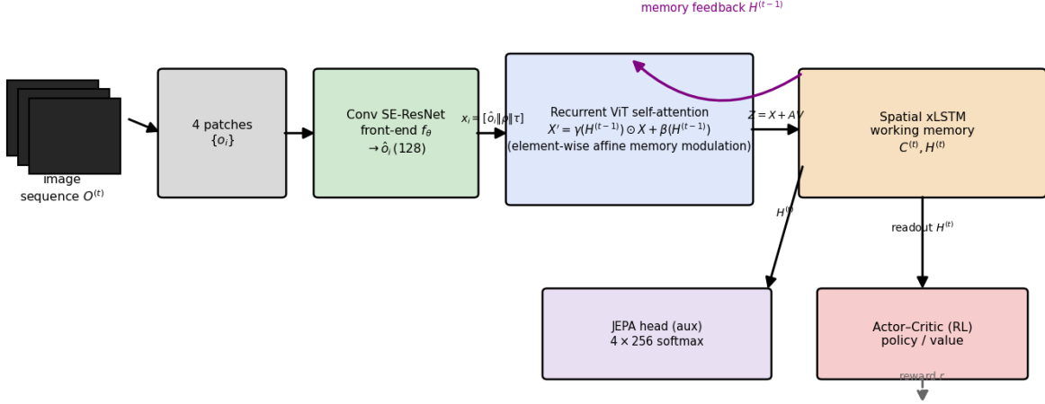
Figure 2 — Recurrent ViT schematic (affine_ew variant)
