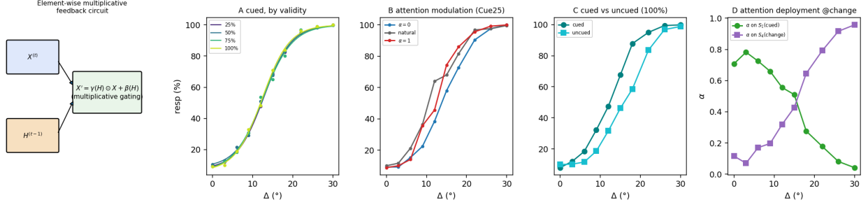
Figure 6: Figs 5–7 analog — feedback mechanism circuit & behaviour. Left: the variant's element-wise multiplicative-gating feedback circuit. A: cued response rate by validity. B: response under enhanced/suppressed attention on the cued change. C: cued vs. uncued at 100%. D: attention deployed on the cued ( S_1 ) vs. change ( S_4 ) location at the change frame vs. \Delta .
