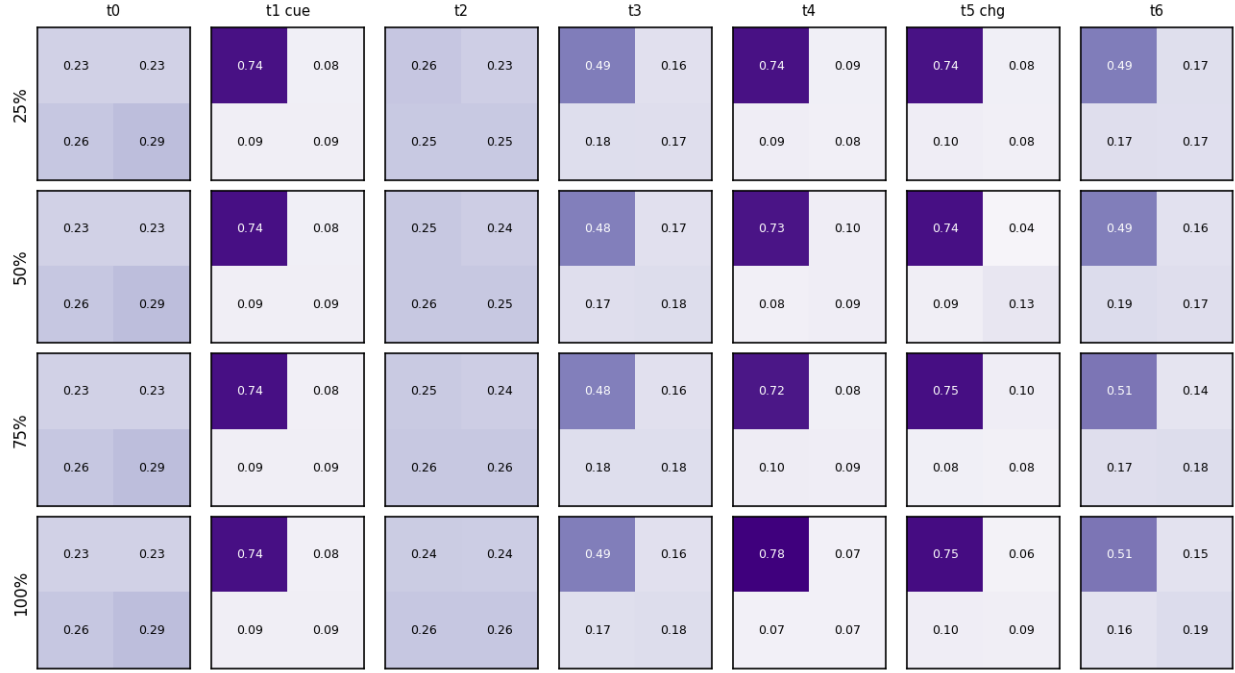
Fig 4A — affine_ew: attention heatmaps per timestep x validity (no-change cue-S1); 2 \times 2 = [[S1, TR], [BL, S4]]
