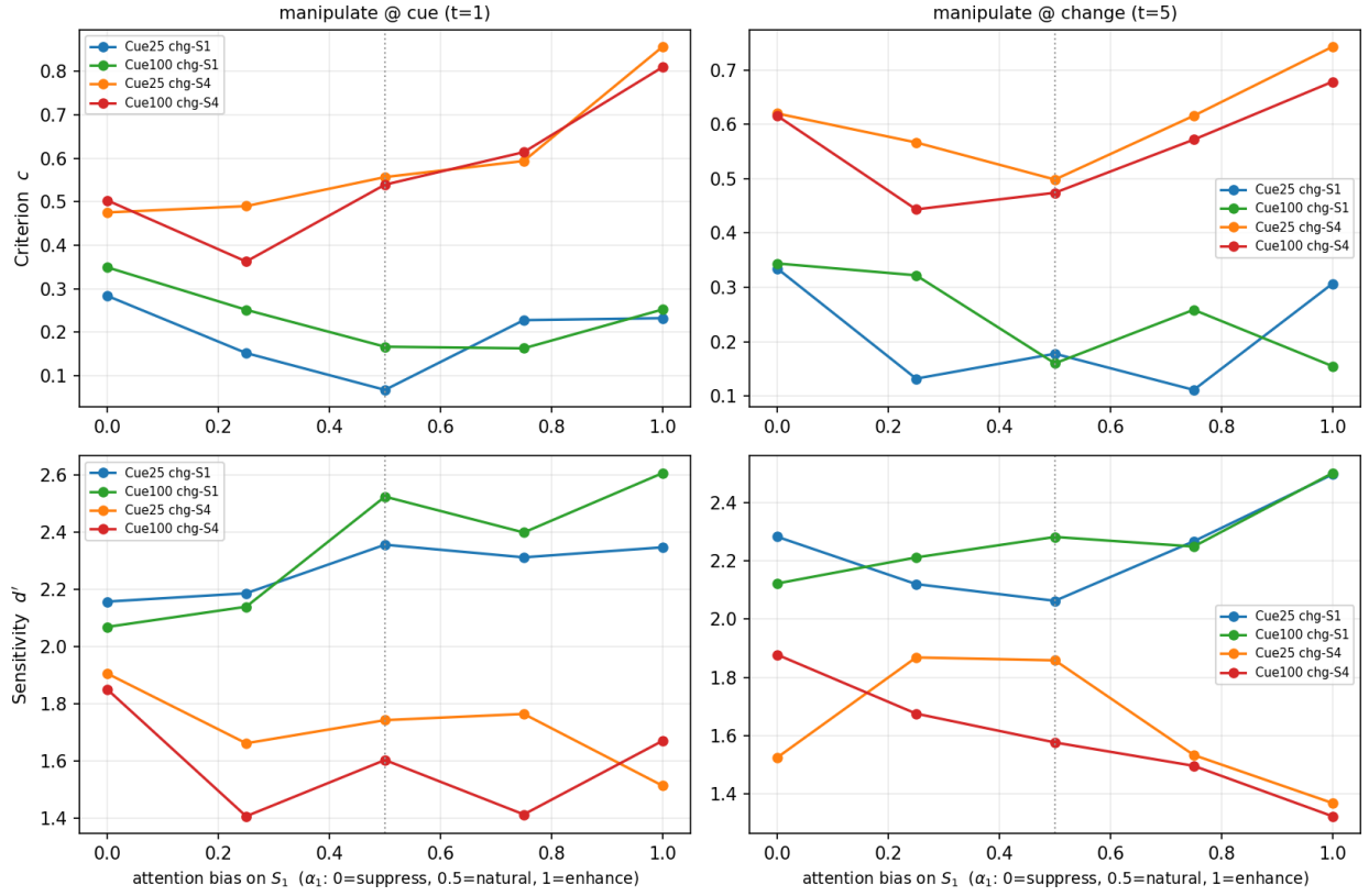
Figure 17: Fig 16 — SDT criterion & sensitivity vs. attention bias on S_1 . Rows: criterion c , sensitivity d' . Columns: manipulate at cue-time ( t=1 ) vs. change-time ( t=5 ). Lines: \{\text{Cue } 25/100\% \} \times \{\text{change at } S_1/S_4\} . \alpha_1=0.5 is natural.
