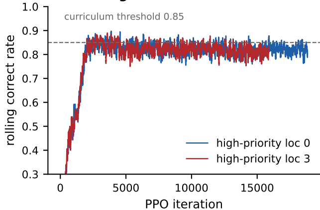
a Learning
