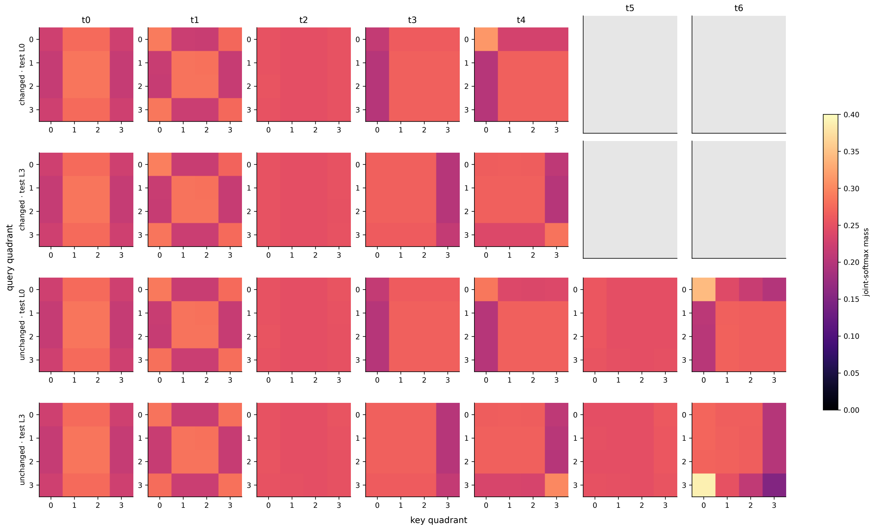
Query-conditioned spatial routing (visual + memory; survivor controlled)
