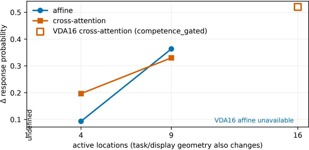
A Valid – invalid response rate ( V=.75 , nearest \Delta=18^\circ )
