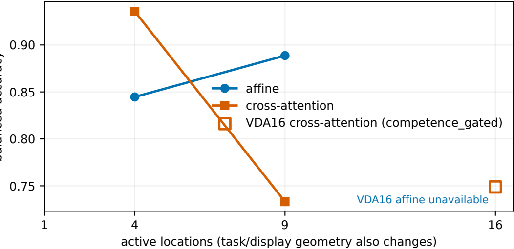
C Final-timestep cued-change decoder
