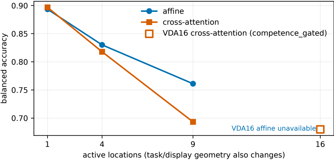
B Final-timestep change decoder
