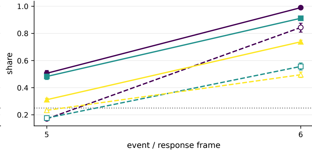
D Affine EW: peak-patch share
