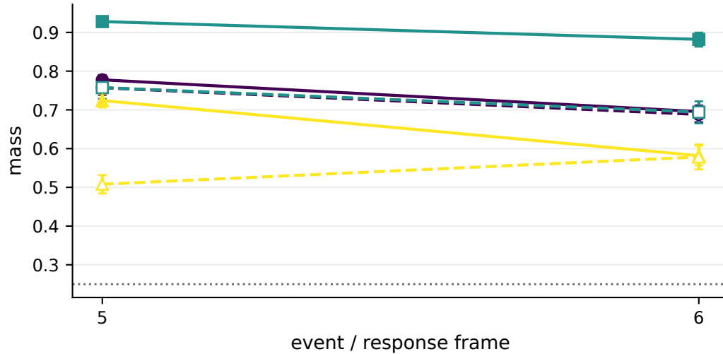
C Affine EW: total quadrant mass
