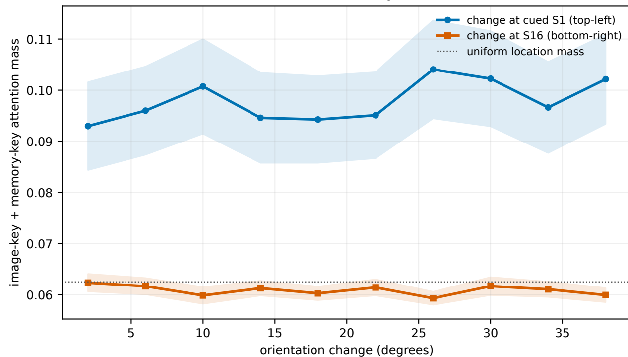
C Achieved attention at changed location on t5
