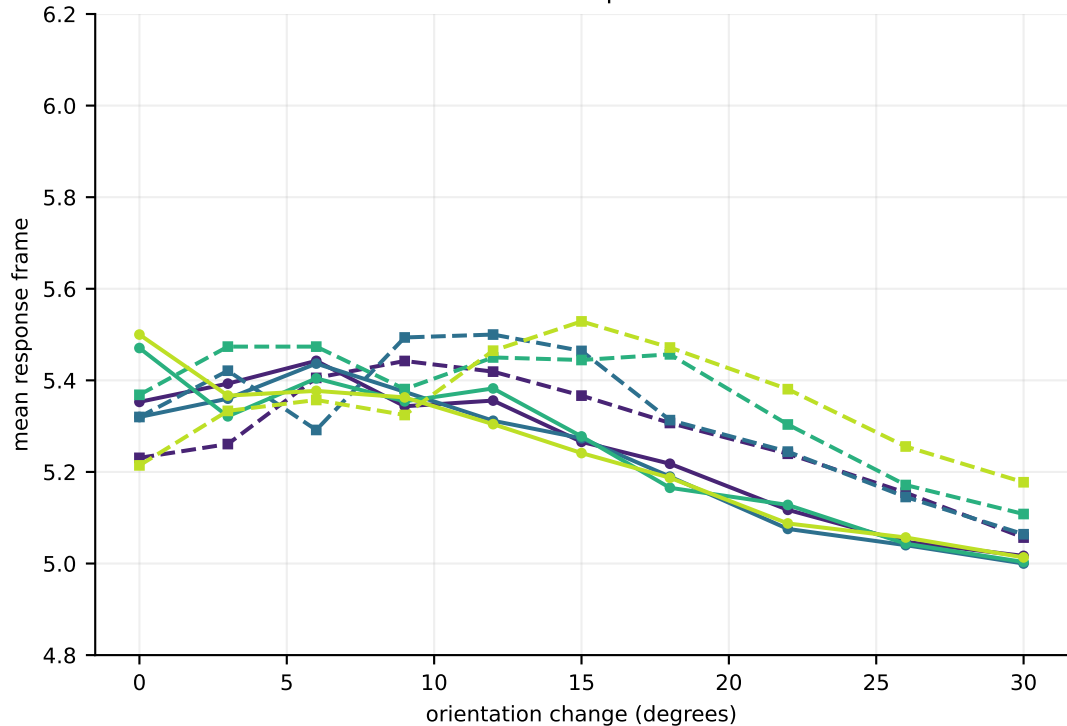
Conditional response time
