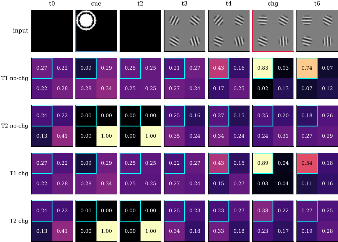
affine_cascade — attention maps, 100% cue@S1 (T1→H1→critic, T2→H2→actor; cyan=cued/changed S1)
