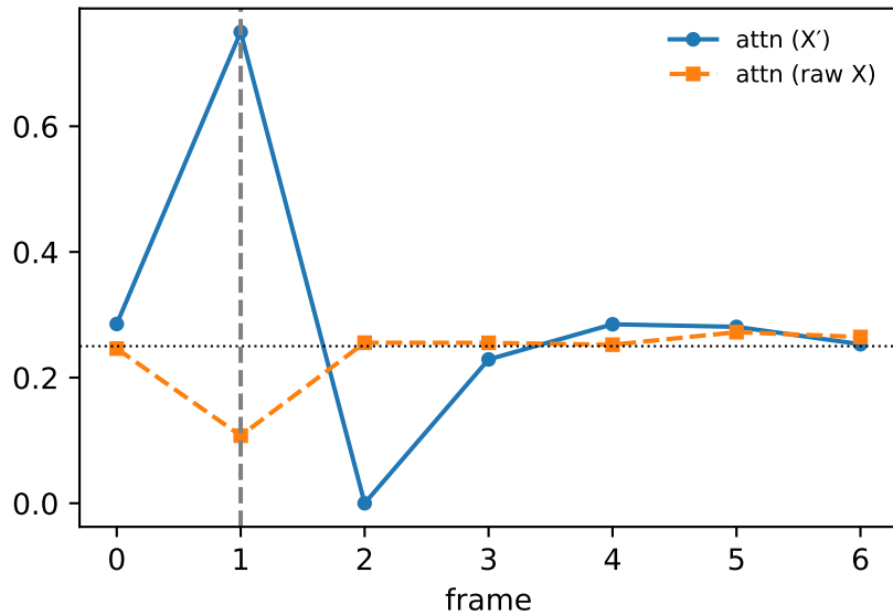
Affine: modulated vs counterfactual
