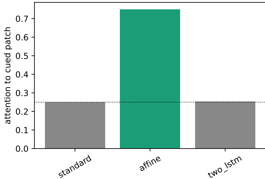
Cue frame (t=1), 100% validity
