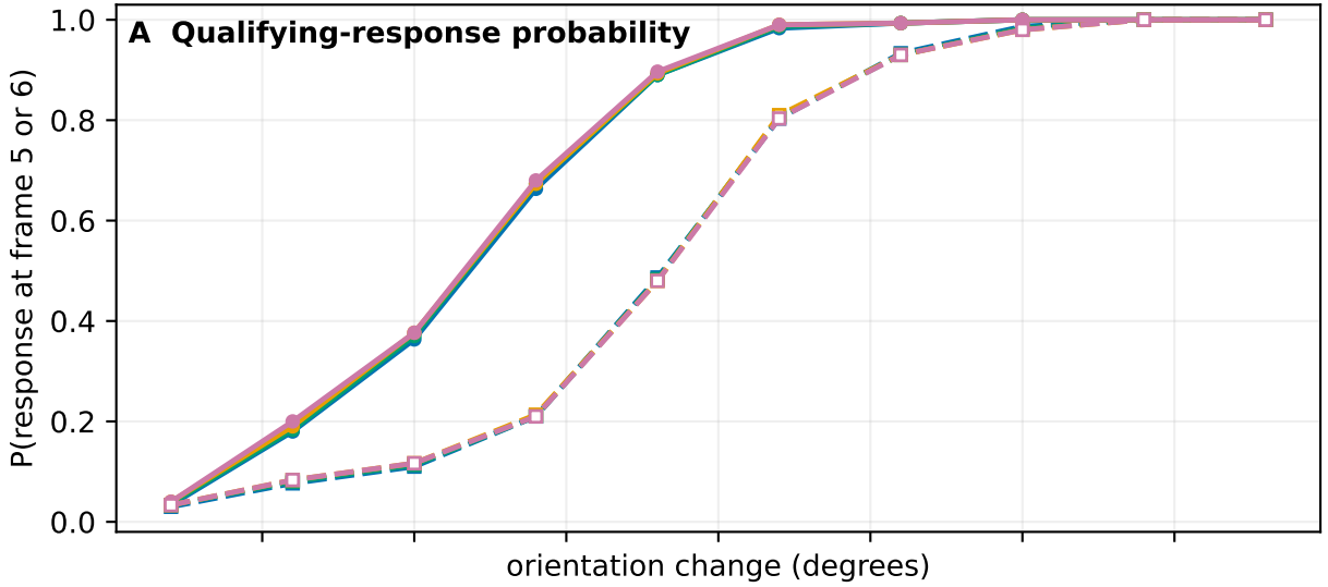
Affine element-wise
