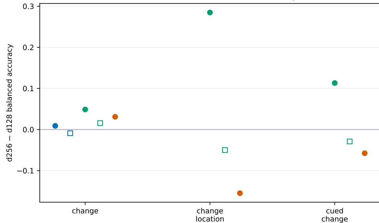
D Invalid-change clamp effect relative to zero bias
