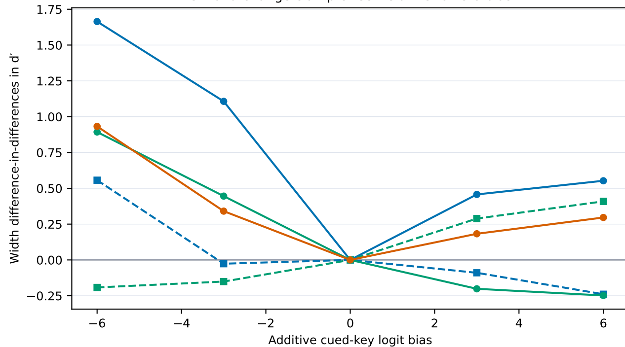
C Valid-change clamp effect relative to zero bias
