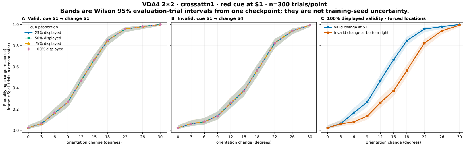
Figure 17: VDA4 cross-attention psychometrics. Checkpoint-recomputed evaluation; 300 trials per point. The all-trial denominator and forced S1-versus-S4 intervention match Figure 16. Separate checkpoints preclude a causal affine-cross-attention contrast.
