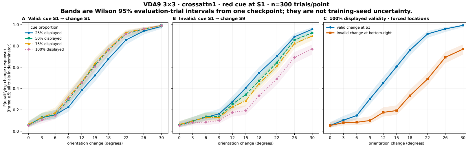
Figure 19: VDA9 cross-attention psychometrics. Checkpoint-recomputed evaluation; 300 trials per point. The lower S9 response at large changes is reproduced in the natural-invalid and forced-invalid panels. It is a verified single-checkpoint result, not a replicated routing effect or evidence of a nine-item capacity boundary.
