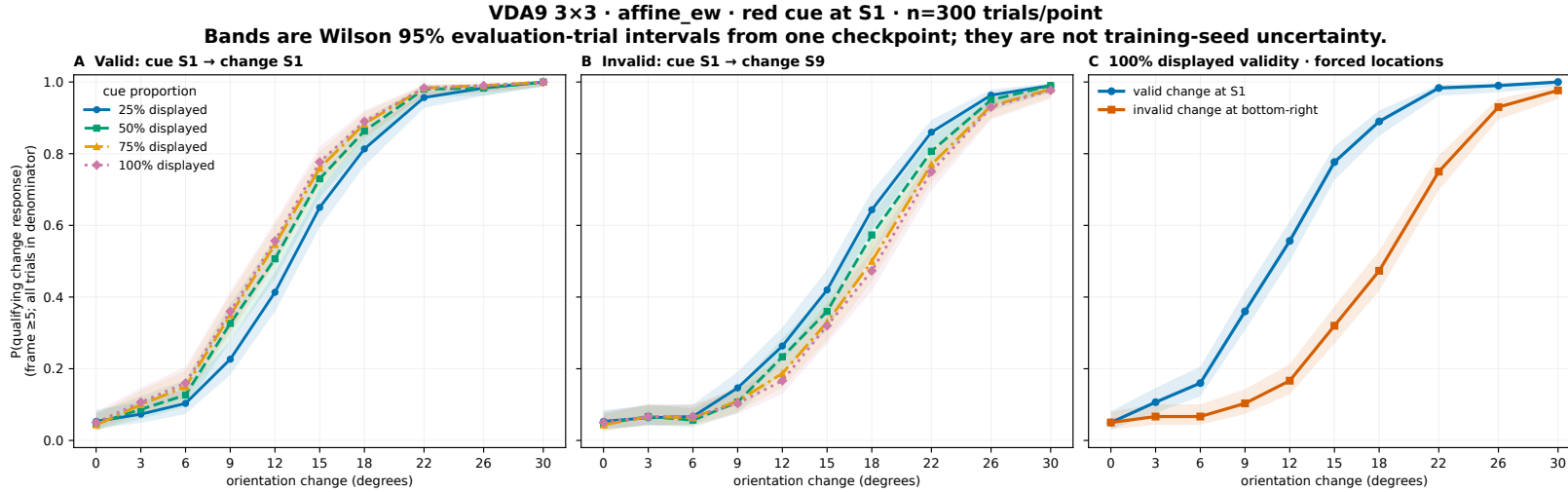
Figure 18: VDA9 affine psychometrics. Checkpoint-recomputed evaluation; 300 trials per point. The invalid location is S9, not a geometry-free “opposing” label. Wilson bands quantify finite evaluation-trial uncertainty only.
