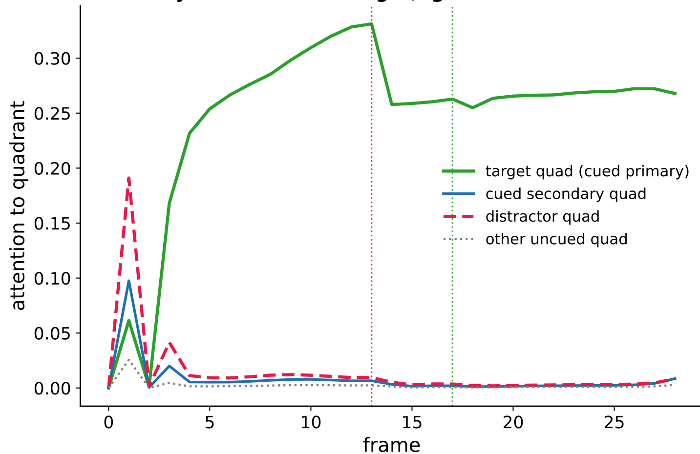
A Priority stream: locks target, ignores distractor
