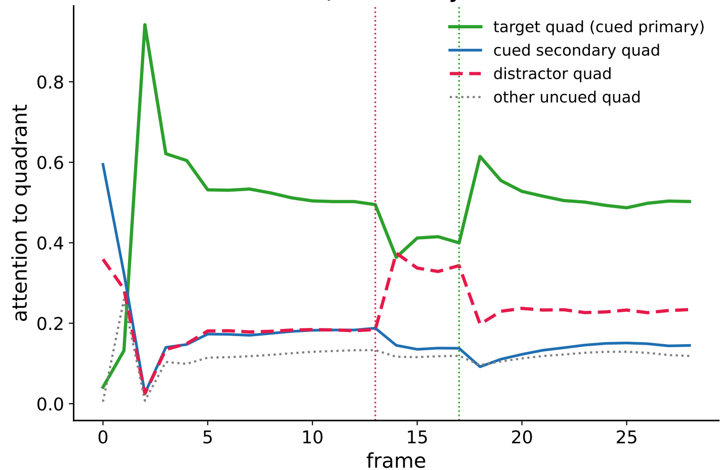
B Value stream: broad, transiently reads distractor
